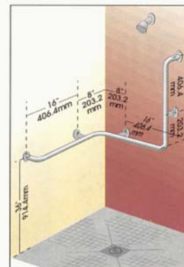
M28 Two Way Shower Safety Rail
